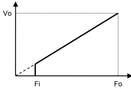
Mode V/F curve
