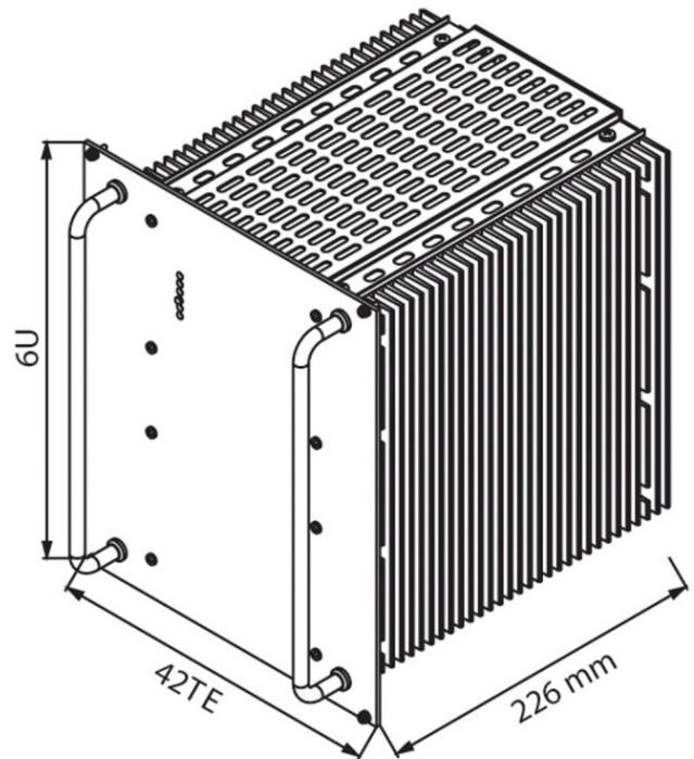
Eurocassette / approx. 10.0 kg (pluggable module for 19" sub-rack)
