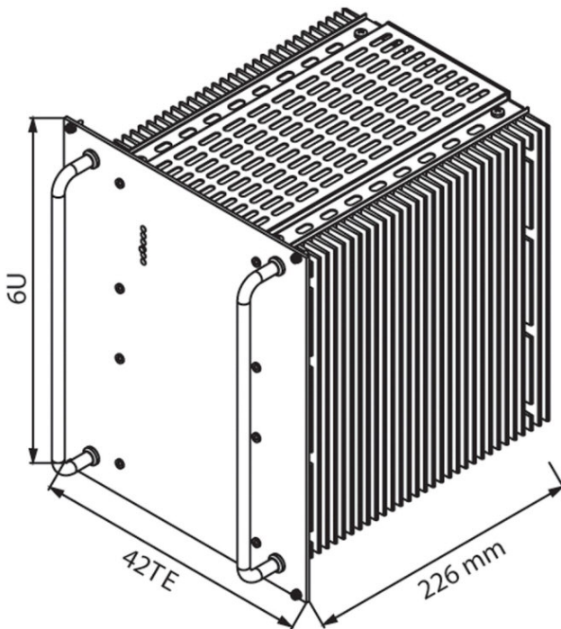
Eurocassette / approx. 10.0 kg (pluggable module for 19" sub-rack)
