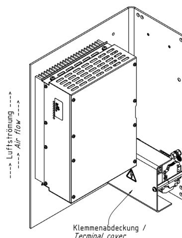
B1591-30-ISOMETRIC
