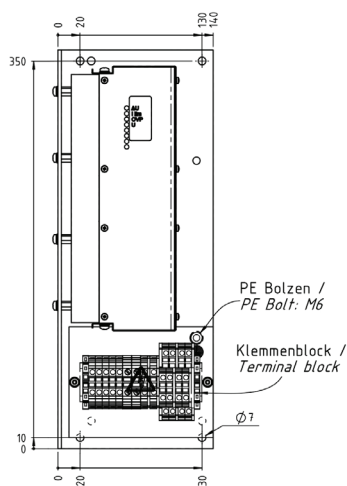
B1591-30-SIDE
