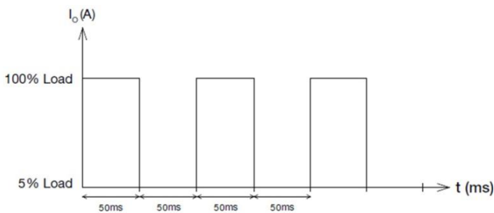
Figure 6. Dynamic Load
