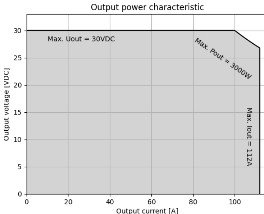
Figure 9.2: Output power DVCH3003-400-24
