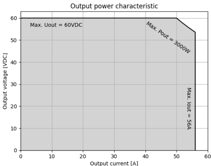
Figure 9.3: Output power DVCH3003-400-48
