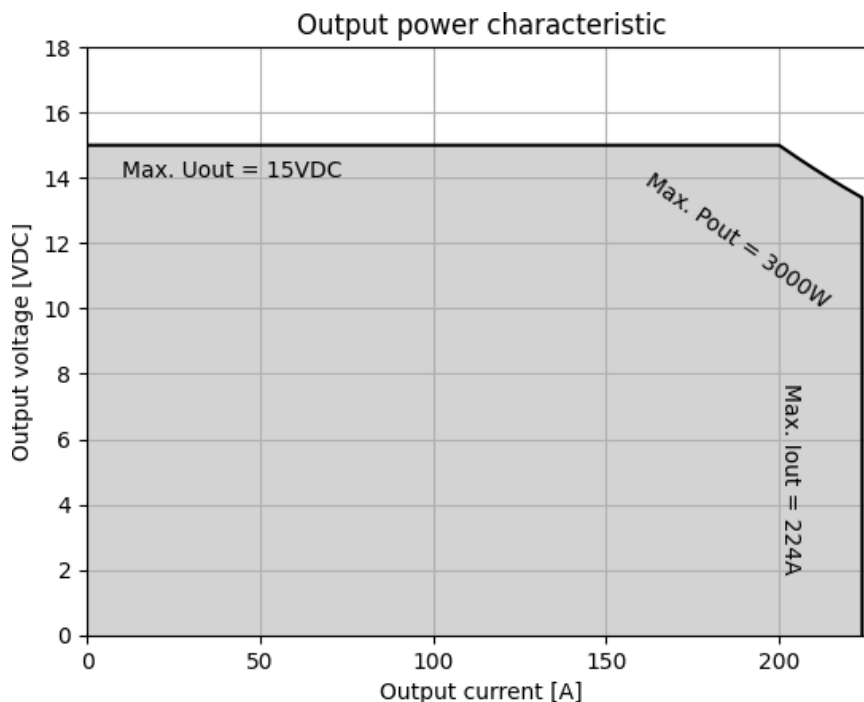
Figure 9.1: Output power DVCH3003-400-12
