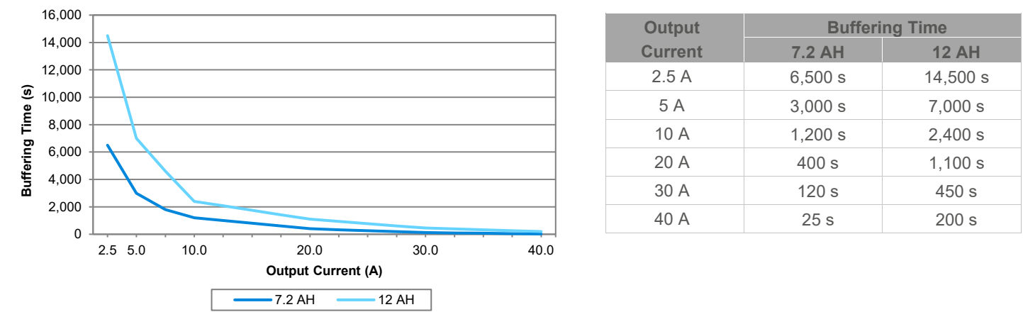
Fig. 1 Buffering Time VS. Output Current
