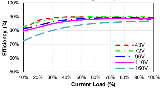
CQB150W-110S28-CMFC Eff Vs Io @25 Deg. C
