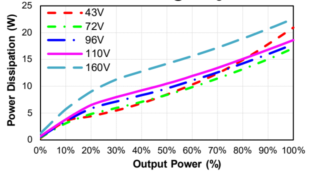
CQB150W-110S28-CMFC Pd Vs Po @25 Deg. C
