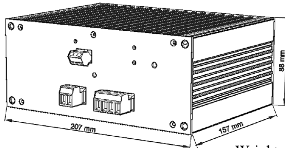
Figure 1. Dimensions
