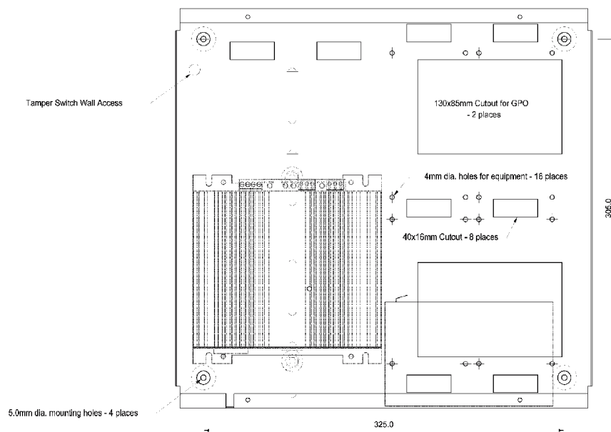
FRONT VIEW - COVER REMOVED (Shows typical installation using PBBS-13-2.5 and 12V 7Ah Battery)
