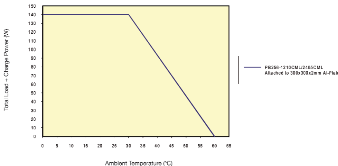
PB256-CML Derating Curves
