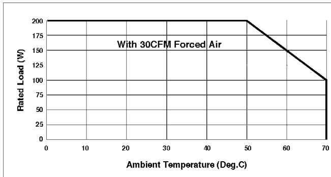
Output Derating Curve
